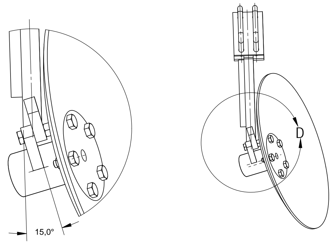
DETAIL D SCALE 1 : 4
